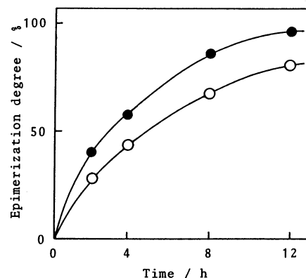
Fig. 1. Time course on epimerization of L-HPG·(±)-PES. The reactions were carried out at 140°C in aqueous solution containing L-HPG·(±)-PES in a sealed tube. Additives: none (○), a 0.1 molar equivalent of DL-HPG (●).
